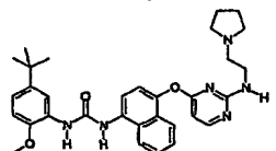
1-(5-tert-Butyl-2-methoxy-phenyl)-3-{4-[2-(2-pyrrolidin-1-ylethylamino)-pyrimidin-4-yloxy]-naphthalen-1-yl}-urea;
